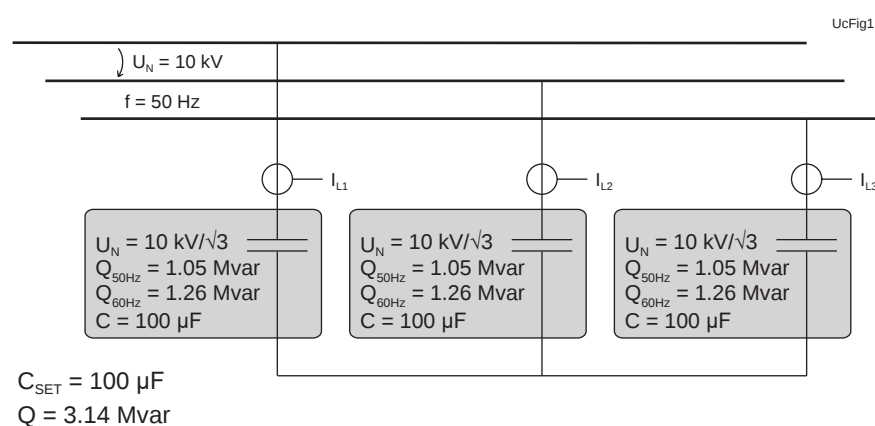
Figure 106 - Capacitor bank built of three single-phase units connected in wye (III Y). Each capacitor is 100 \mu F and this value is also used as the setting value.
