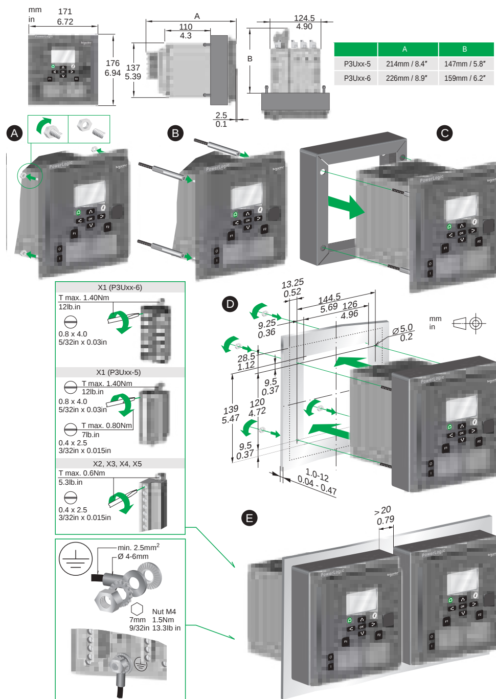
Figure 193 - Panel mounting with the raising frame REL52834
