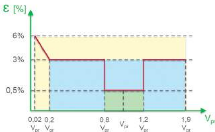
Figure 251 - Magnitude accuracy
