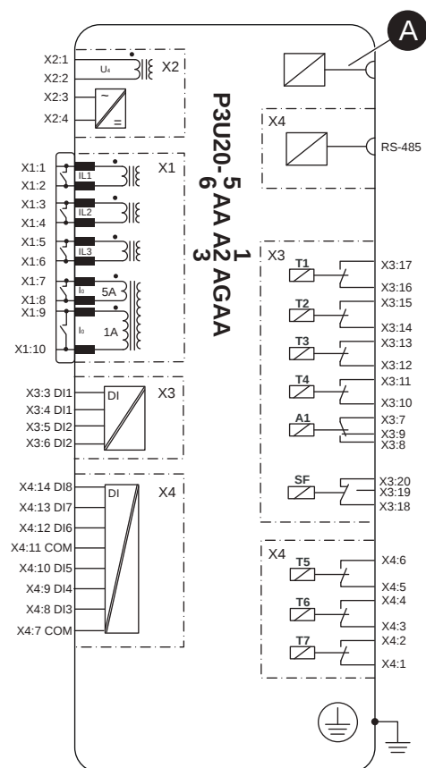
Figure 210 - P3U20 5AA A1AGAA block diagram
