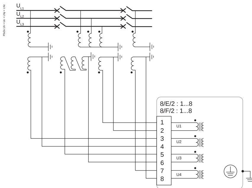
Figure 283 - LN+U 0 +LNy+LNz
