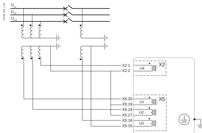
Figure 276 - 3LN+LNy
