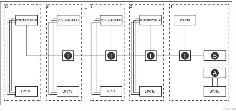
Figure 264 - LPVT sharing application without test sockets/plugs
