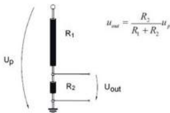
Figure 258 - Resistive divider
