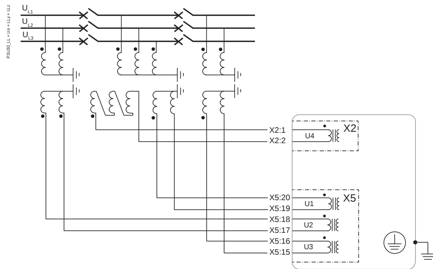
Figure 280 - LL+U 0 +LLy+LLz
