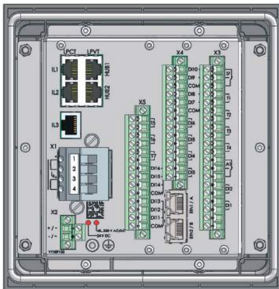
Figure 229 - P3U rear panel – LPIT
