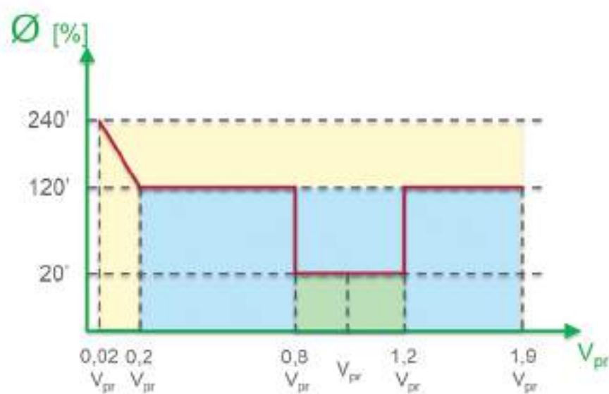
Figure 252 - Phase accuracy
