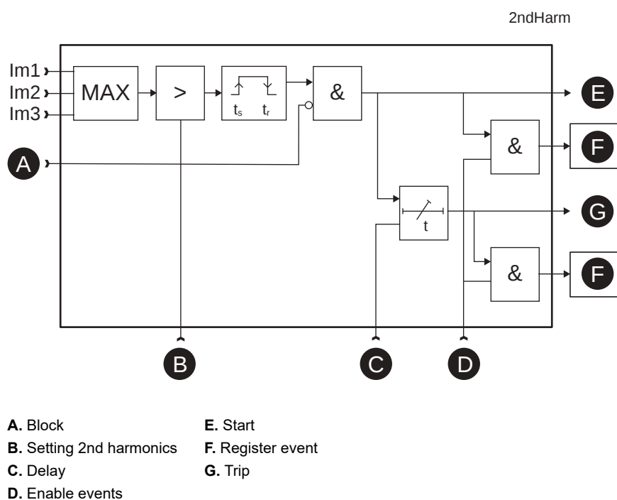
Figure 125 - Block diagram of the magnetizing inrush detection stage
