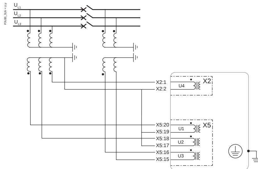
Figure 275 - 3LN+LLy
