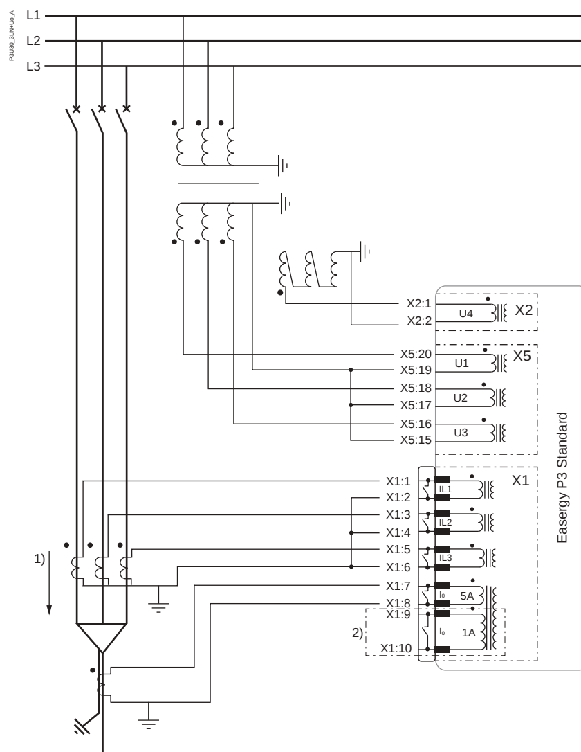
Figure 225 - 3LN voltages + U o + 3LN currents + core balance EF
