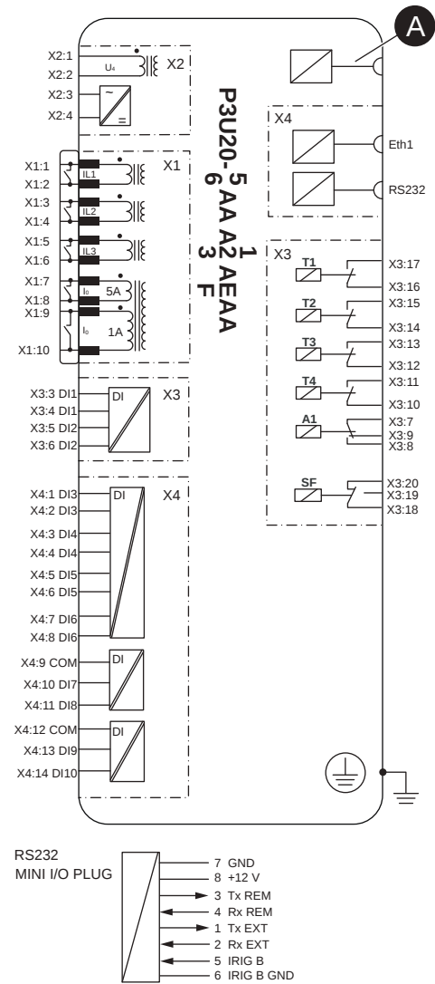
Figure 208 - P3U20 5AA A1AEAA block diagram
