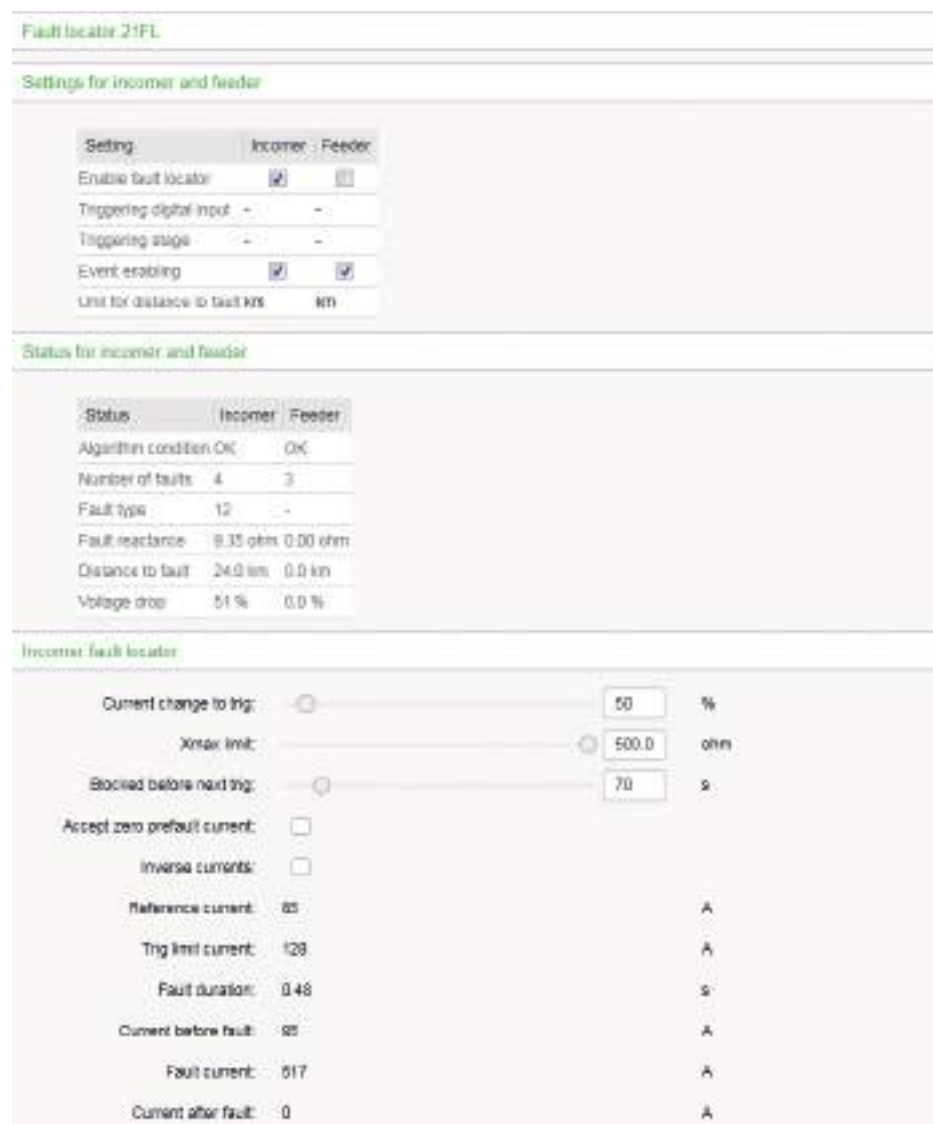
Figure 157 - Application example with fault location algorithm at the feeder side
