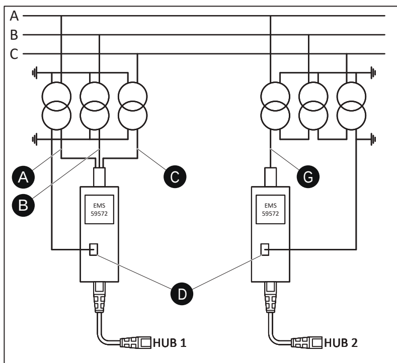
Figure 233 - 3LN+U 0 connection
